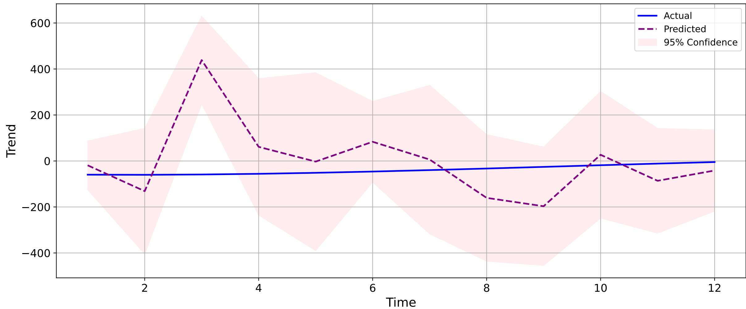
Backdoor-ALL - Testing
